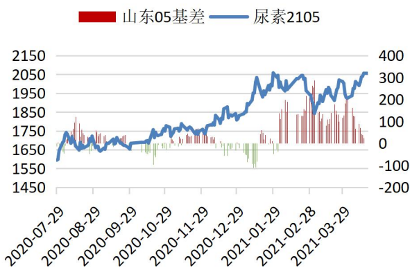
UR2105基差
